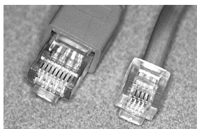
FIGURE 221. RJ-45 connector ( left ) and RJ-11 connector ( right )
