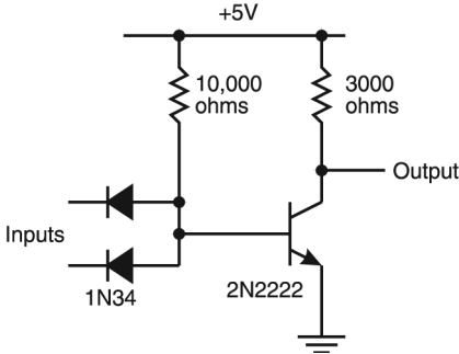
FIGURE 160. NAND gate built with transistors and diodes
