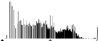
FIGURE 130. Histogram
