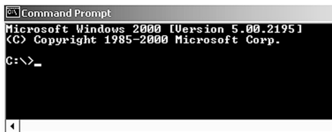
FIGURE 62. Command prompt
