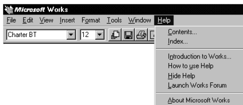
FIGURE 206. Pull-down menu
