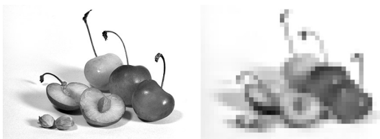
FIGURE 198. Pixelated image
